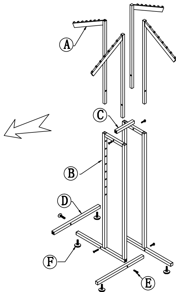
ASSEMBLY EXPLODED VIEW
