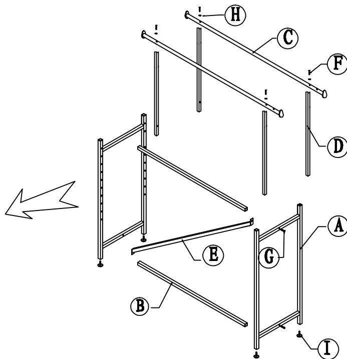
ASSEMBLY EXPLODED VIEW
