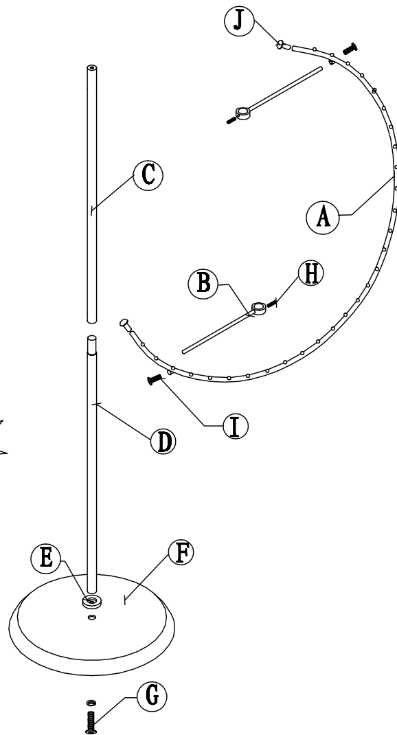
ASSEMBLY EXPLODED VIEW
