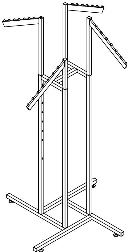
ASSEMBLING DRAWING
