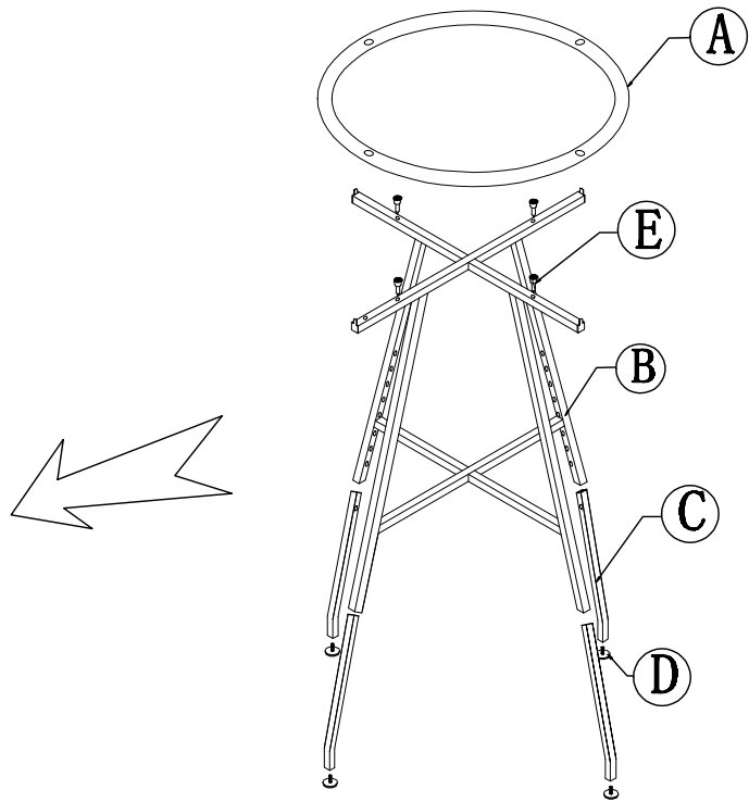
ASSEMBLY EXPLODED VIEW
