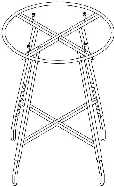
ASSEMBLING DRAWING
